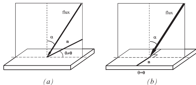
Figure 4. Irradiation geometry and LC alignment in the first (a) and second (b) modes.
